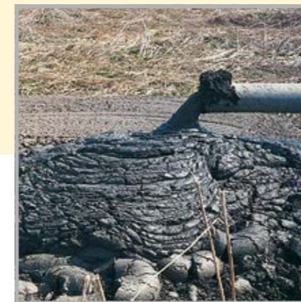
River sludge with high dry solids content has short drying times
